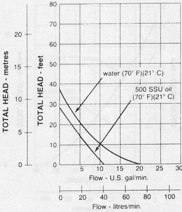
Pump tube with air motor operating at 80 (5.5 bar) psi inlet air pressure to motor.
