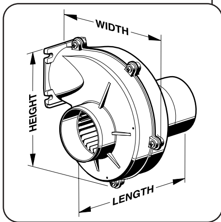
Flangemount
