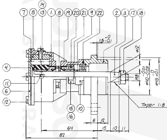
F4B-9 Impeller pump Art. No. 10-24335-01
